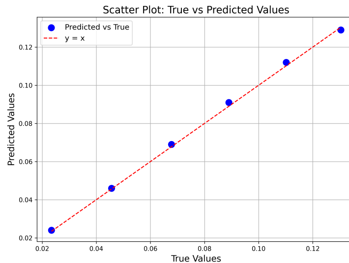
Figure 3: Scatter plot comparing the true values of \Upsilon(t) obtained from analytical methods with the predicted values generated by the machine learning model
