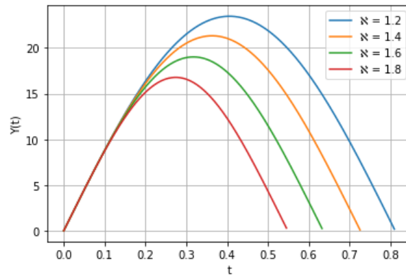
Figure 1: The solution behavior of Example 1
