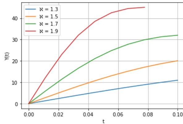
Figure 2: The solution behavior of Example 2
